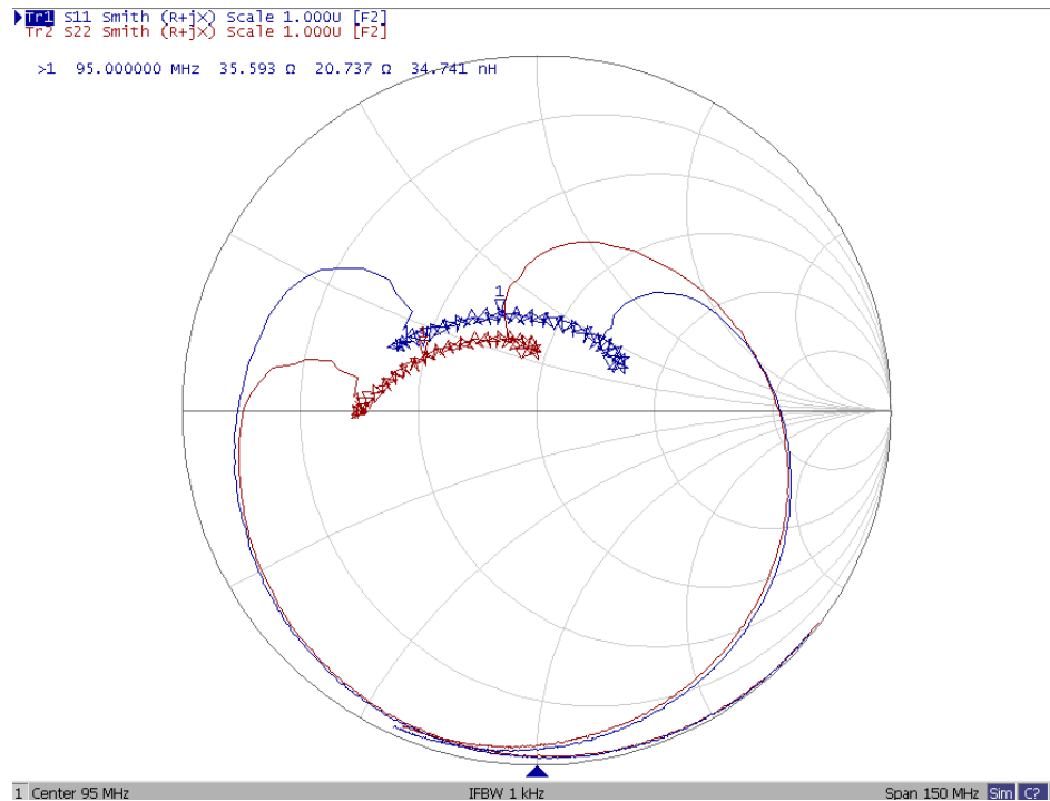
Fig3. Horizontal: 4MHz/Div Vertical: 1dB/Div
