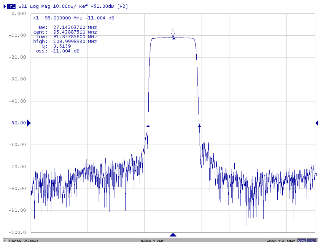
Fig1. Horizontal: 15MHz/Div Vertical: 10dB/Div
